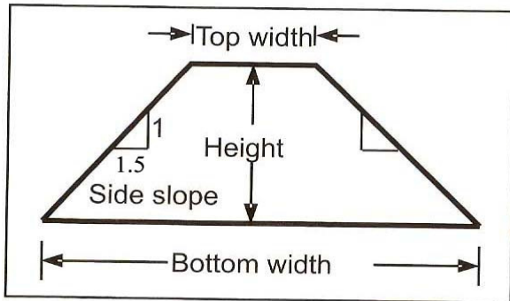
Cross-section of a contour bund
