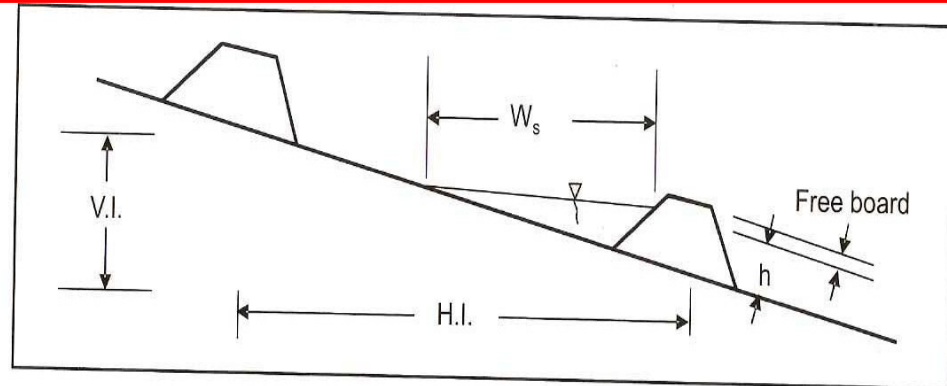
Definition sketch for a contour bund
